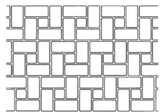
Flanders Weave (194mm x 90mm)
